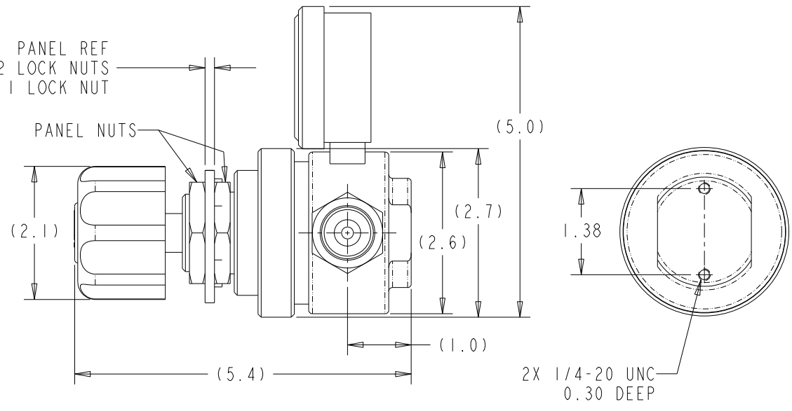
PANEL CUT-OUT
