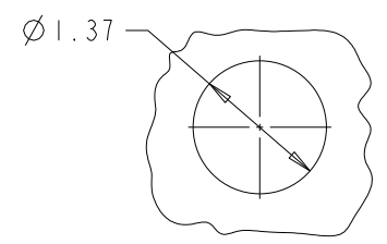
PANEL CUT-OUT
